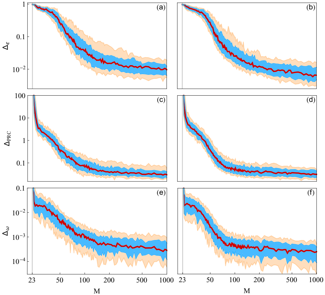
FIG. 5. Error of the reconstruction in dependence on the number of interspike intervals M used for the analysis. Panels (a, c, e) and (b, d, f) show the results for PRC type I and PRC type II, respectively. Panels (a, b) show the error of the coupling coefficients \varepsilon_i Eq. (7), panels (c, d) the error of the PRC Eq. (8) and panels (e, f) the error of the frequency \omega Eq. (9). For each value of M reconstruction error was computed for 6000 different networks. The blue (dark gray) and the orange (light gray) areas contain 50% and 75% of the errors, respectively; the median is shown in red (bold line).
