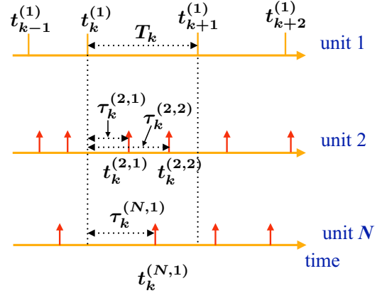
FIG. 2. Illustration of notations used. T_k is an interspike interval of the driven unit. \tau_k^{(i,l)} is the time (relative to the beginning of the interval T_k ) when the spike number l from the unit number i arrives.
