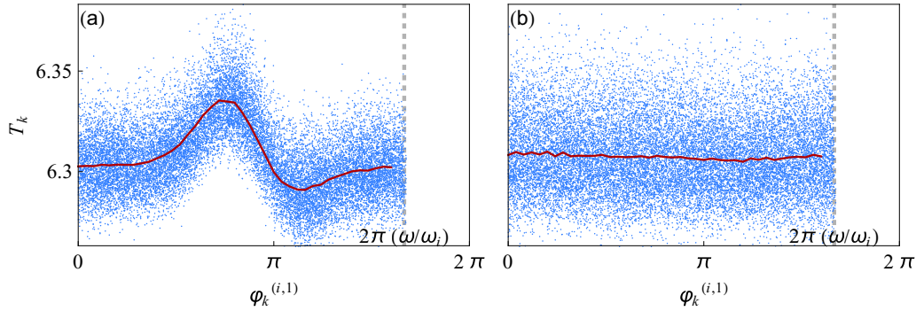
FIG. 7. Scatter plots of interspike intervals T_k vs. approximated phase \varphi_k^{(i,1)} of the first spike from a chosen driving oscillator i , for a strong coupling strength (a) and for a weak one (b). The horizontal axis is divided into N_b = 50 bins and solid red curve shows the average of T_k over each of the bins, \bar{T}_n^{(i)} , as a function of the central phase \bar{\varphi} of the bins; 2 \times 10^4 interspike intervals are used in this computation.
