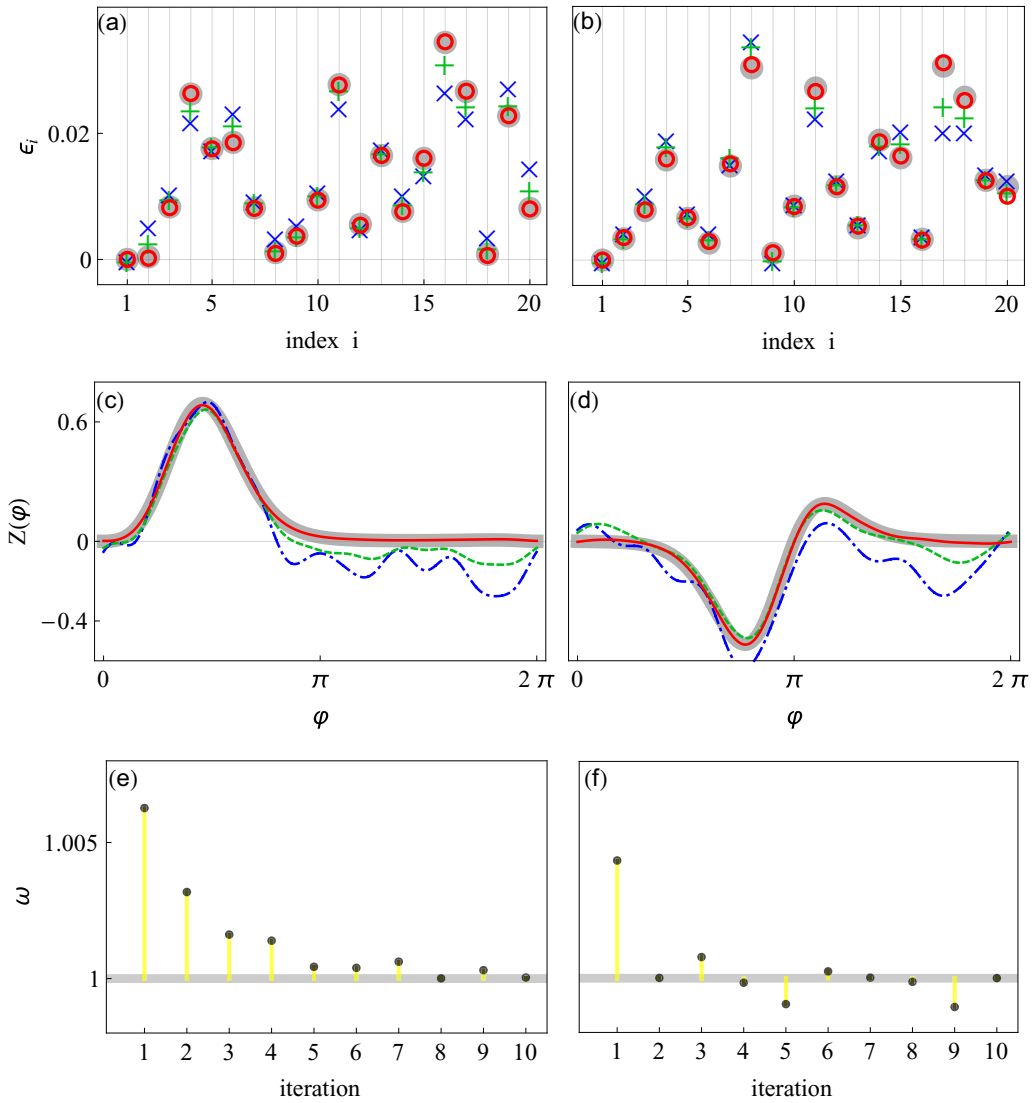
FIG. 3. Reconstruction of a network of 20 units using M = 200 interspike intervals. Panels (a, c, e) and (b, d, f) show the results for PRC type I and PRC type II, respectively; see Eqs. (1) and (2). (a, b) Strength of incoming connections for the first oscillator: true values (gray disks) and values recovered after 1, 2, and 10 iterations (blue crosses, green pluses, and red circles, respectively). (c, d) True (wide gray curve) and reconstructed PRCs, after 1, 2, and 10 iterations (blue dashed-dotted, green dashed, and red solid curves, respectively). (e, f) Estimated natural frequencies as functions of the iteration number; the true value \omega = 1 is shown by horizontal gray line. Notice that in this figure we illustrate the most difficult case of the slowest node.
