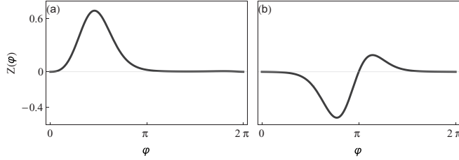
FIG. 1. Model phase response curves of type I (a) and type II (b).
