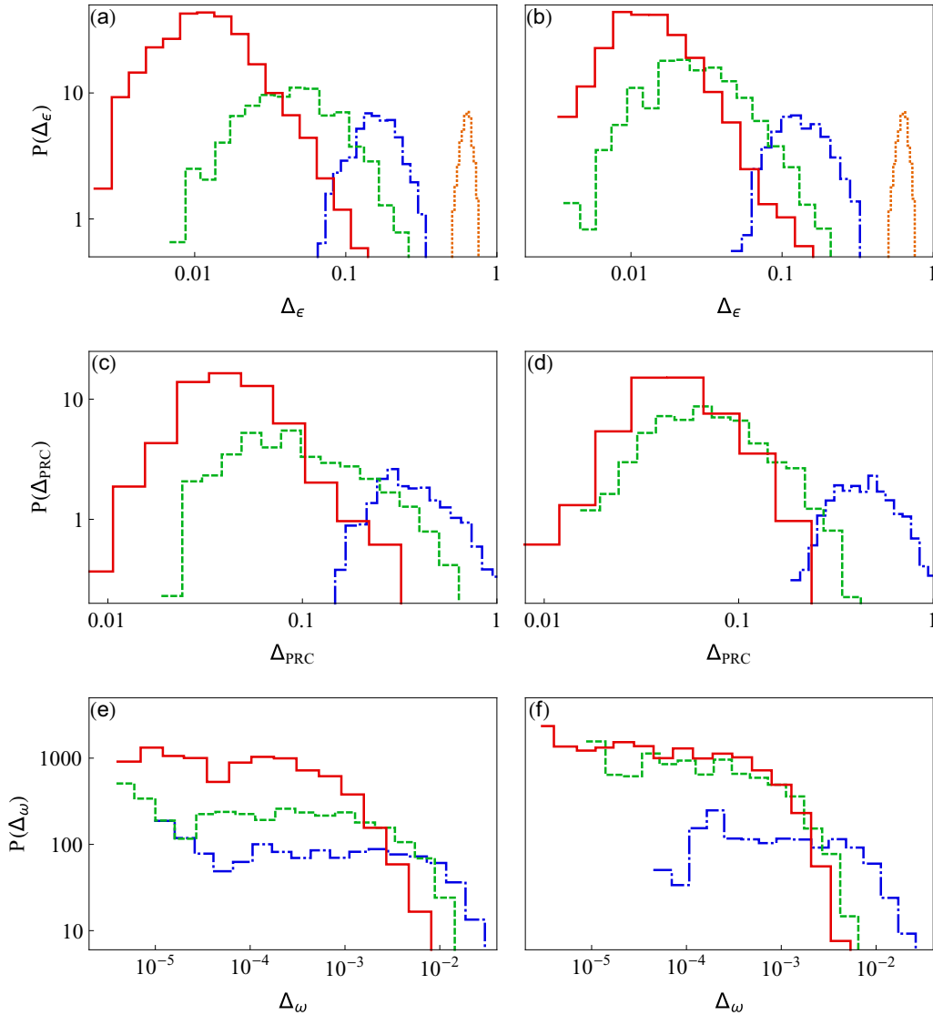
FIG. 4. Histograms of errors of the coupling strengths \Delta_\varepsilon (a, b), PRC \Delta_{\text{PRC}} (c, d), and frequency \Delta_\omega (e, f); see Eqs. (7)–(9). Panels (a, c, e) and (b, d, f) correspond to tests with PRC type I and type II, respectively. In each panel, the results of the first, third, and tenth iterations are shown in blue (dash-dotted), green (dashed), and red (solid line), respectively. In (a, b) also the distribution of errors for initial values \varepsilon_i = 1 is shown in orange (dotted line).
