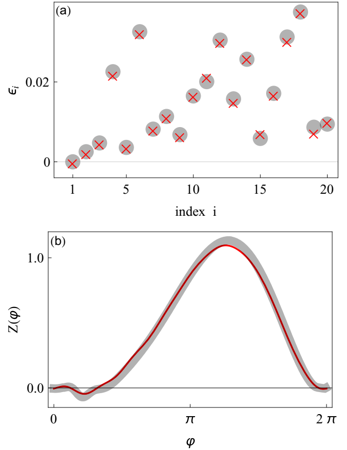
FIG. 6. Reconstruction of a network of 20 Morris-Lecar neuronal oscillators; see Eqs. (10)–(12). 200 interspike intervals were used for the reconstruction. (a) True values of the strength of the incoming connections for the first neuron (gray disks) and these values reconstructed after 10 iterations (red crosses). (b) True (wide gray curve) and reconstructed (solid red curve) PRC. Notice that in this figure we illustrate the most difficult case of the slowest node.
